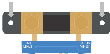
Top view SmartShunt IP65 indicating mounting holes and side view SmartShunt indicating mounting method.
