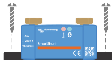
Top view SmartShunt IP65 indicating mounting holes and side view SmartShunt indicating mounting method.
