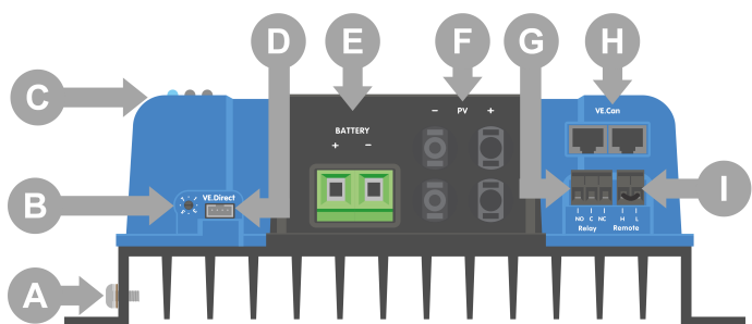
70 A MC4-model.
