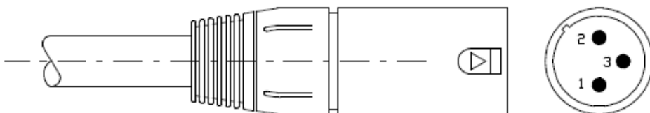
Figure 1 XLR-connector
