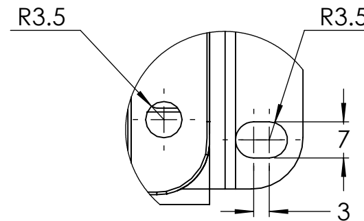
DETAIL A 4x SCALE 1 : 1
