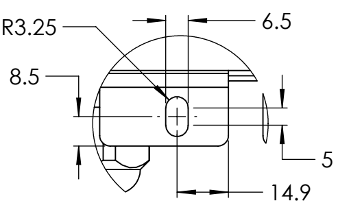
DETAIL A SCALE 2 : 3
