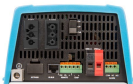
Connection area MultiPlus 500VA
