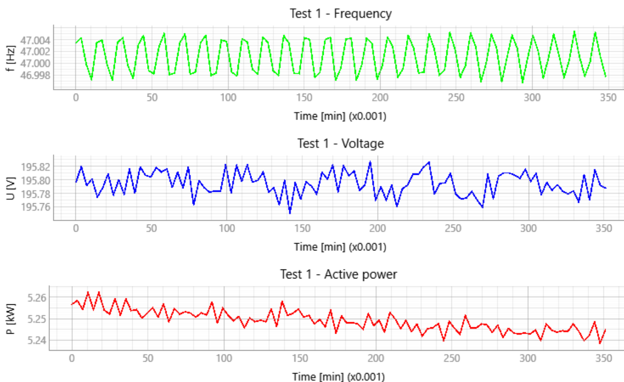
Test 1 - Frequency, Voltage, active power over time diagram
