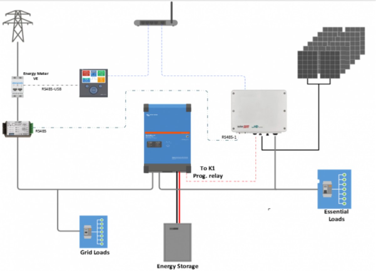
Configuration example 2: Use of Internal programmable relay K1, See Figure 2
