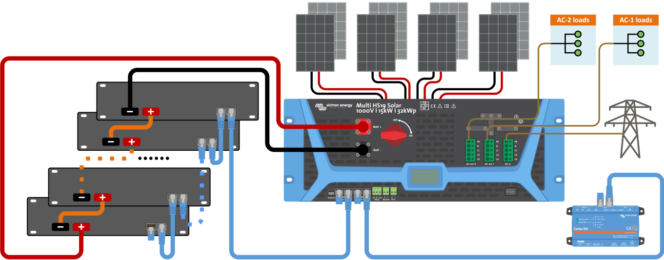
Multiple batteries in series
