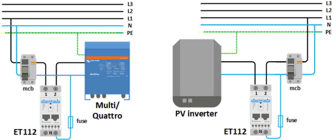
Wiring when used as a grid meter. Wiring when used to measure PV inverter or AC Genset.
